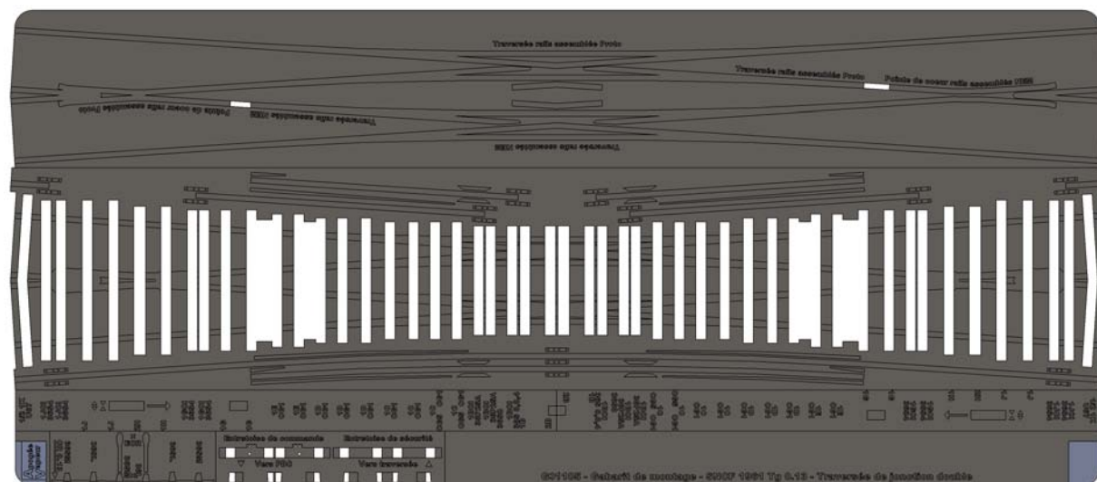
Gabarit G31105 (Ech 1/2)
