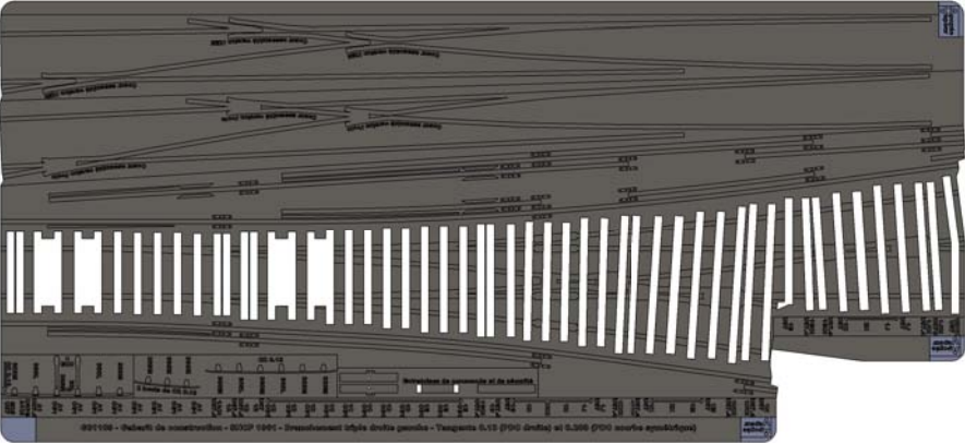
Gabarit G31109 (Ech 1:3)
