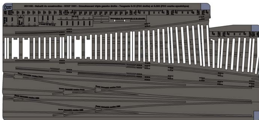
Gabarit G31108 (Ech 1:3)
